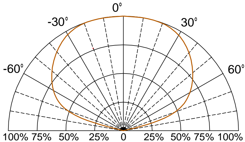
Fig.6 Directivity Radiation
