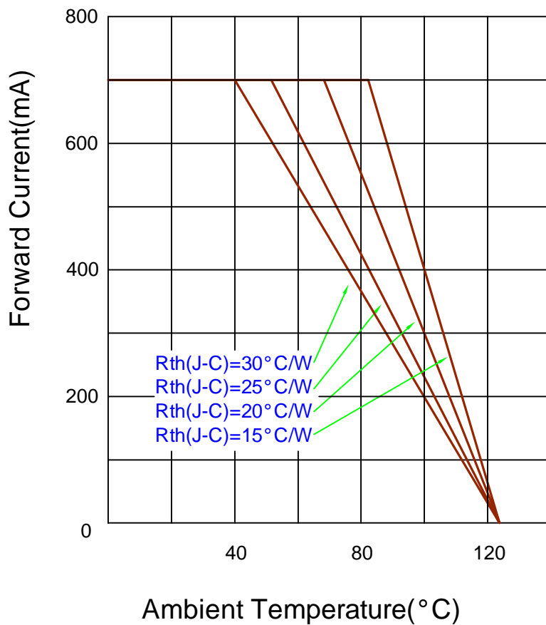
Fig.2 Operating current vs. Ambient Temperature
